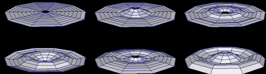
Ripples traveling across a pond
