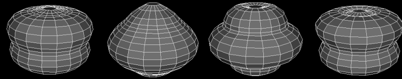
Hemisphere inverting due to opposing impulses applied to the equator and pole
