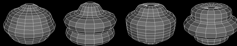
Response of a sphere vibrated sinusoidally at the poles
