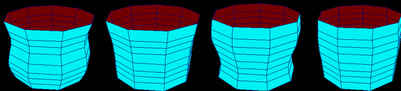
Traverse waves traveling down a cylinder
