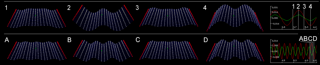
Standing waves in a plane at two different frequencies
