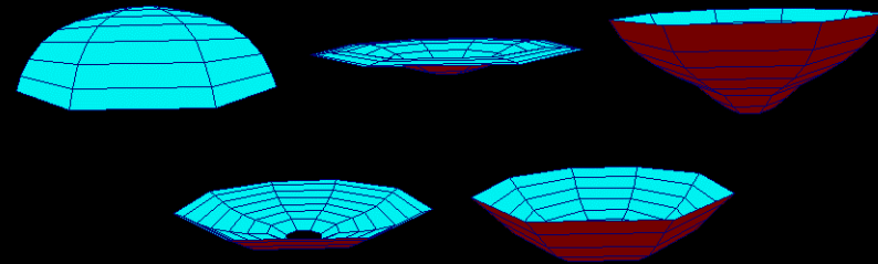
Hemisphere inverting due to opposing impulses applied to the equator and pole
